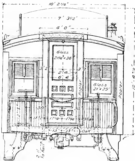
Fig. 489. End Elevation.
